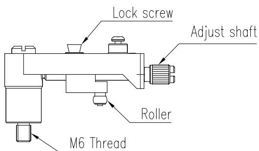
图7-2: 直行程跨度件装配
