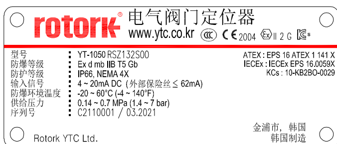
图L-26: YT-1050 Ex d mb IIB T5 Gb (CCC)
