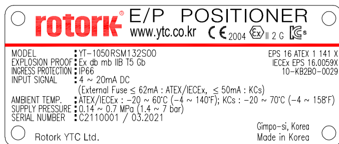
图L-23: YT-1050 Ex db mb IIB T5 Gb (ATEX, IECEx, KCs)
