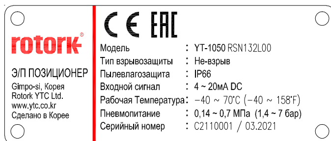
图L-22: YT-1050 Non-explosion (EAC)
