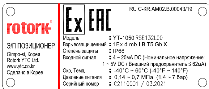
图L-25: YT-1050 1Ex d mb IIB T5 Gb X (EAC)
